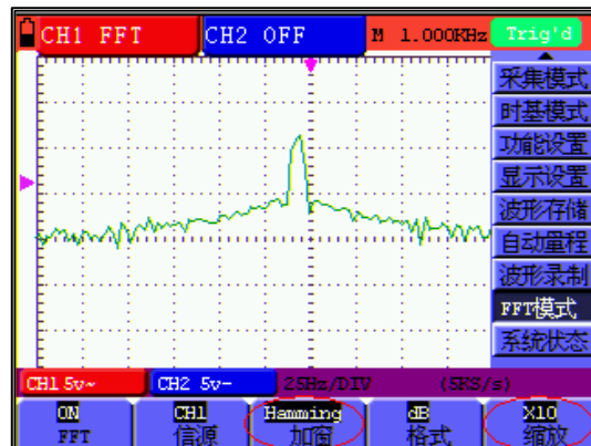
圖64. HAMMING窗
