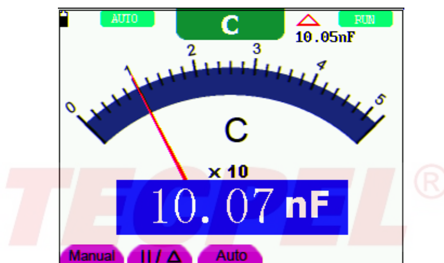
Figure 24: Capacitance Measurement
