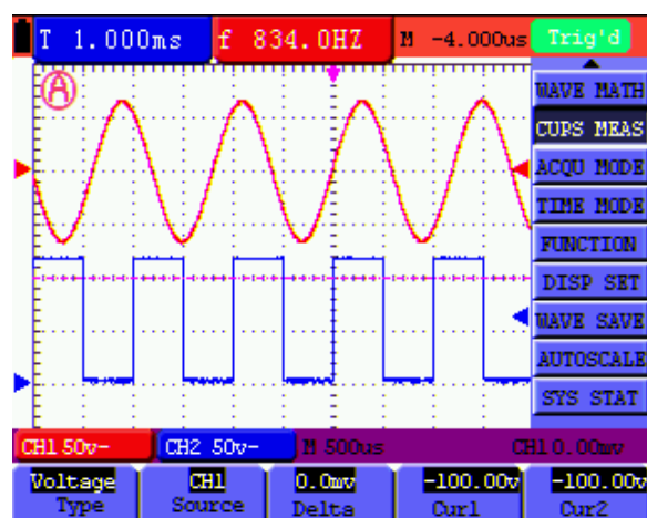
Figure 52 : Use the Cursor for a Voltage Measurement
