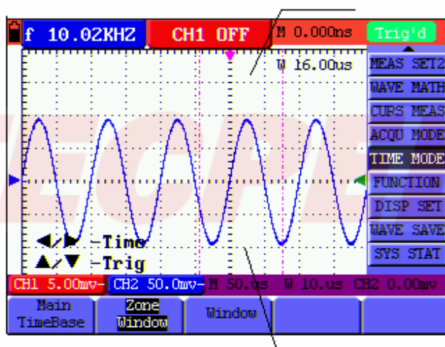
Figure 67: Window Setting
