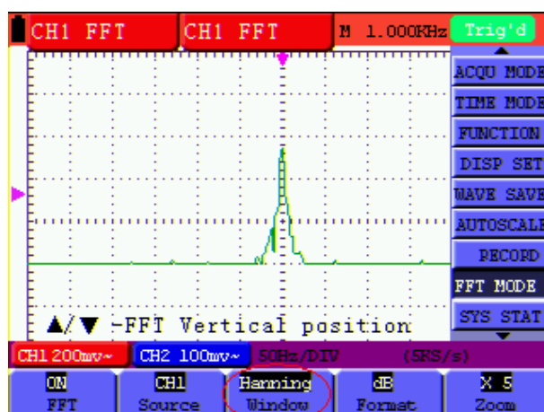
Fig.63 . Hanning window
