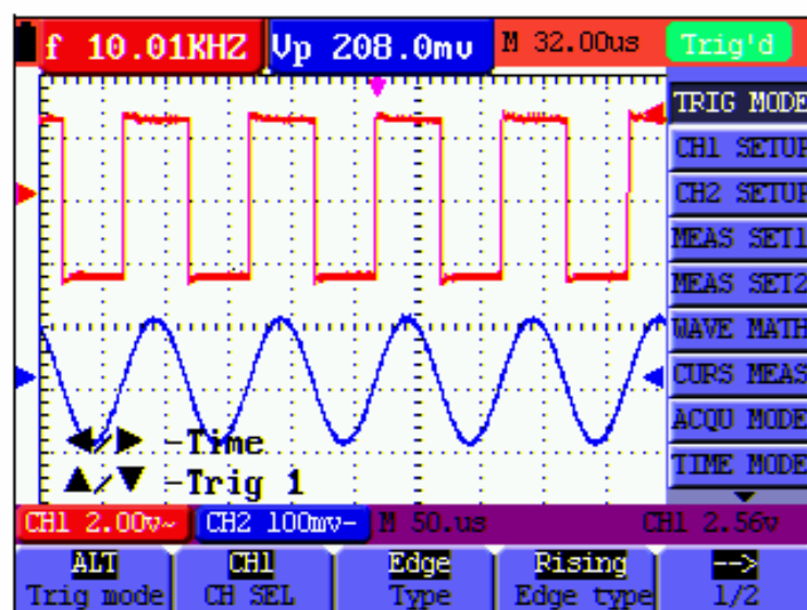
Figure 44 Alternate Trigger
