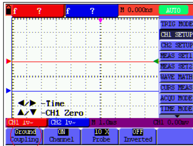
Figure 37: Ground Coupling
