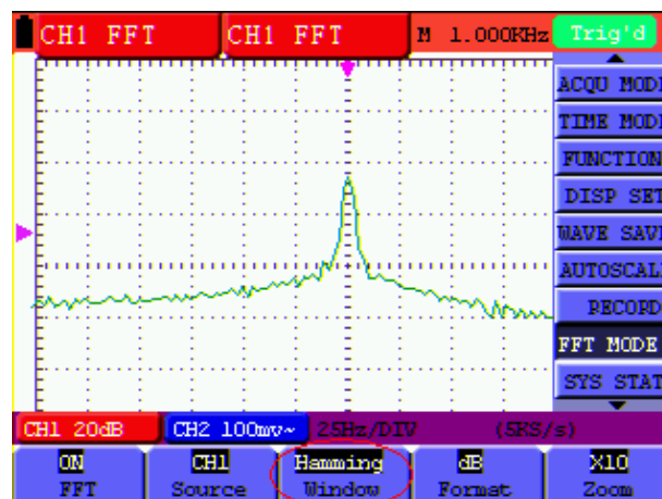
Fig.64. Hamming window
