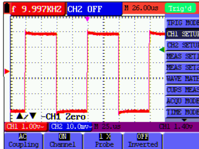
Figure 17: AC-Coupling
