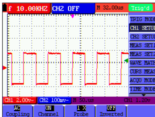
Figure 35: AC Coupling
