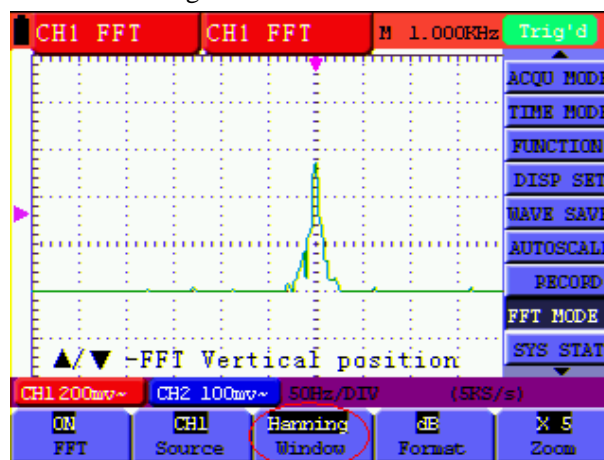
Fig.63. Hanning window
