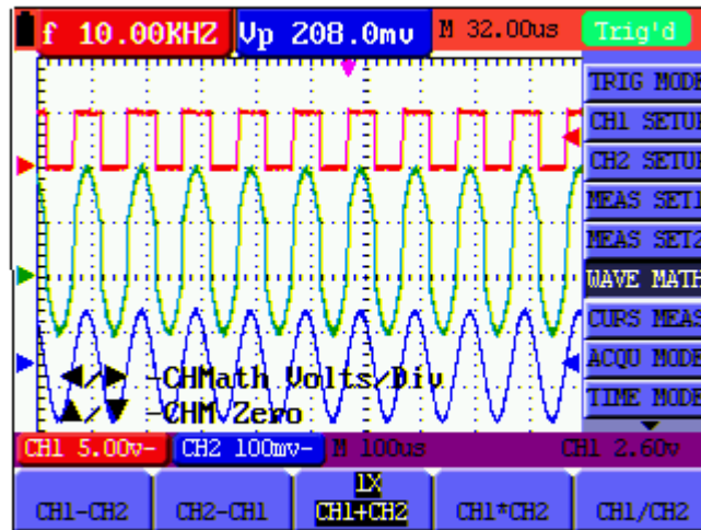
Figure 38: Waveform Mathematics
