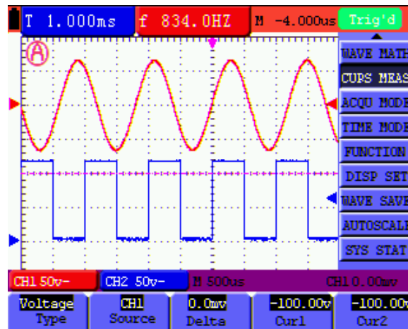
Figure 52: Use the Cursor for a Voltage Measurement
