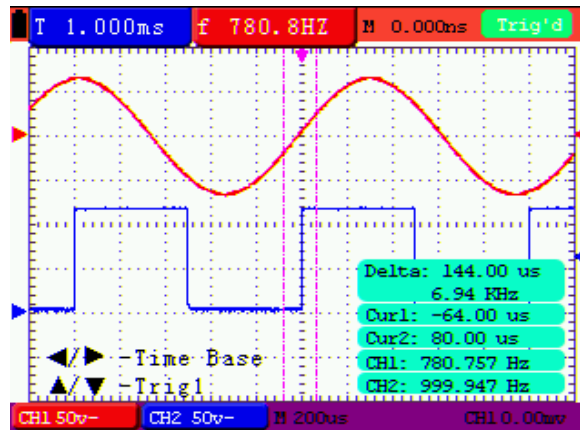
Figure 55: Use the Cursor for a Time Measurement
