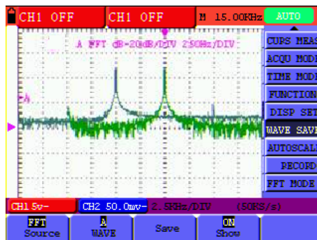
Figure 50: Waveform Saving in FFT Mode
