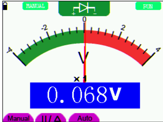
Figure 22: Diode Measurement
