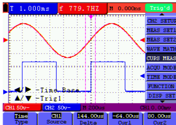
Figure 54: Cursor time measurement
