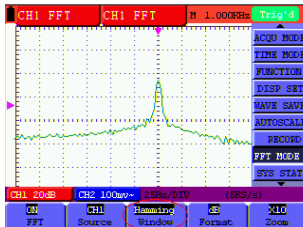
Fig.64. Hamming window
