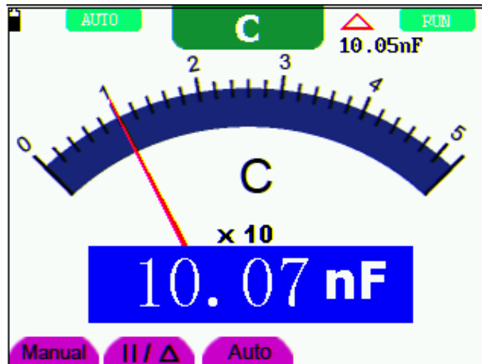
Figure 24: Capacitance Measurement
