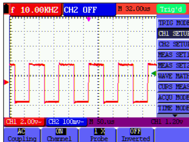
Figure 35: AC Coupling
