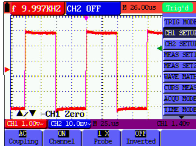
Figure 17: AC-Coupling
