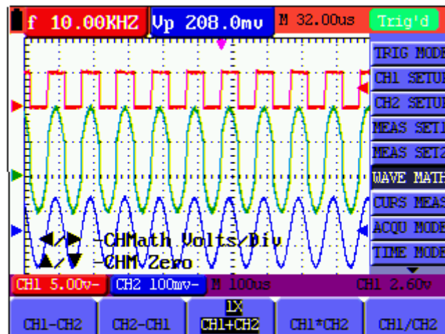
Figure 19: Waveform Mathematics
